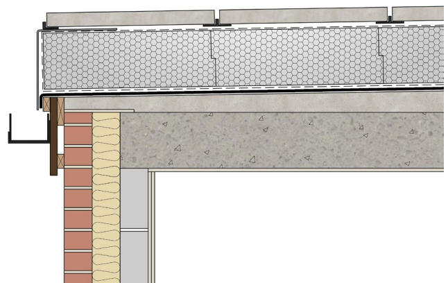
Figure 7. Ballasted inverted roof – detail at eaves
